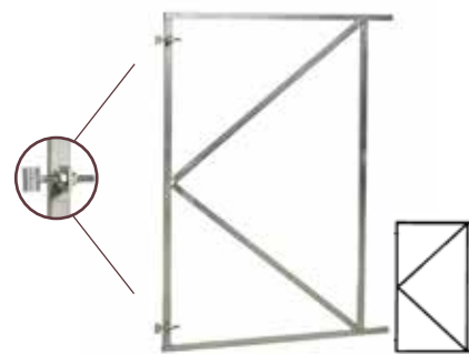
Verstelbaar poortframe - verzinkt 100x80 cm - 2 ogen Q003014 €56,72 p/st 90x155 cm - 2 ogen Q003005 €68,75 p/st 100x155 cm - 2 ogen Q003006 €70,28 p/st 110x155 cm - 2 ogen Q003007 €76,28 p/st 120x155 cm - 3 ogen Q003008 €79,35 p/st 130x155 cm - 3 ogen Q003009 €84,19 p/st 140x155 cm - 3 ogen Q003010 €87,24 p/st 150x155 cm - 3 ogen Q003011 €90,29 p/st
